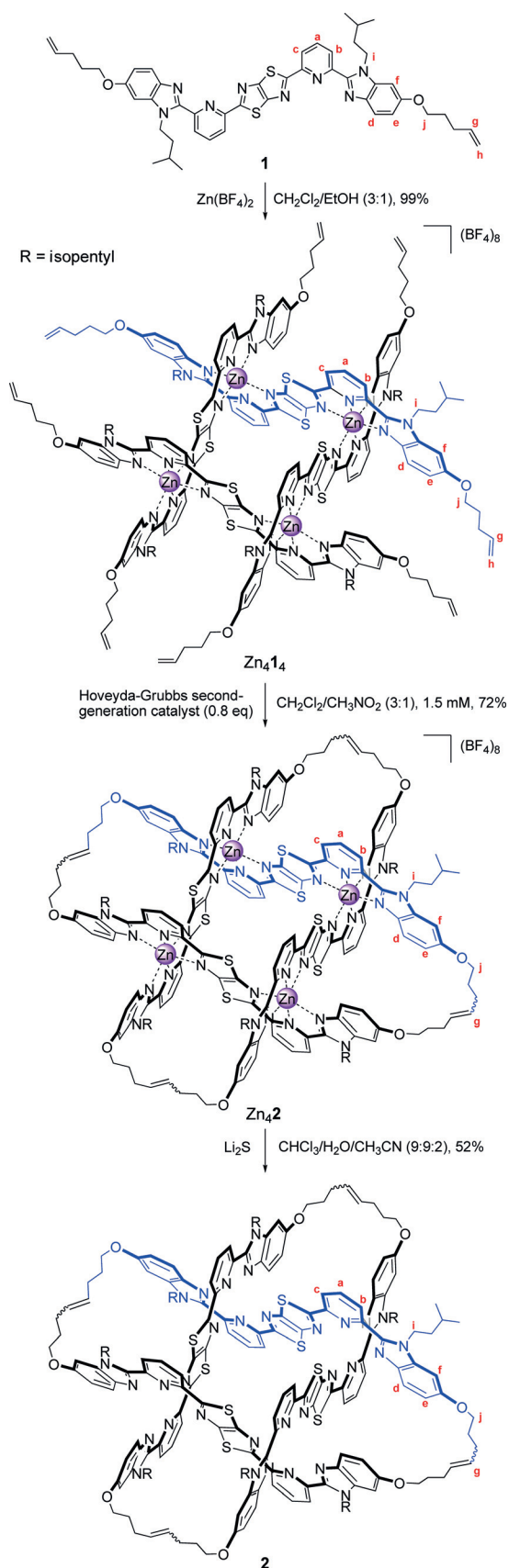
Scheme 1. Synthesis of interwoven grid [\text{Zn}_4\text{14}](\text{BF}_4)_8 and Solomon links [\text{Zn}_4\text{2}](\text{BF}_4)_8 and 2 .
