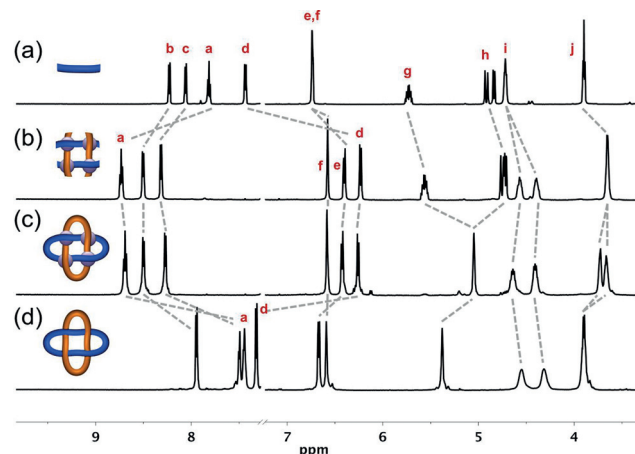
Figure 2. Partial ^1\text{H} NMR spectra (2:1 \text{CDCl}_3/\text{CD}_3\text{CN} , 600 MHz, 298 K except for (d)) of a) ligand 1 , b) grid complex [\text{Zn}_4\text{14}](\text{BF}_4)_8 , c) Solomon link [\text{Zn}_4\text{2}](\text{BF}_4)_8 , and d) demetalated Solomon link 2 (325 K). Proton assignments refer to the labeling in Scheme 1.
